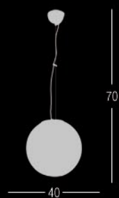
1911-20 1xE27 Max.40W
