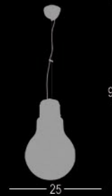
1940-1 1xE27 Max.40W
