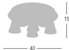
2040-6 ARM 30W LED
