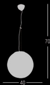
1911-30 1xE27 Max.40W
