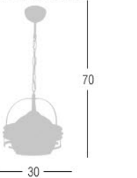
1712-1 SP 1712-1 BP 1xE27 Max.60W
